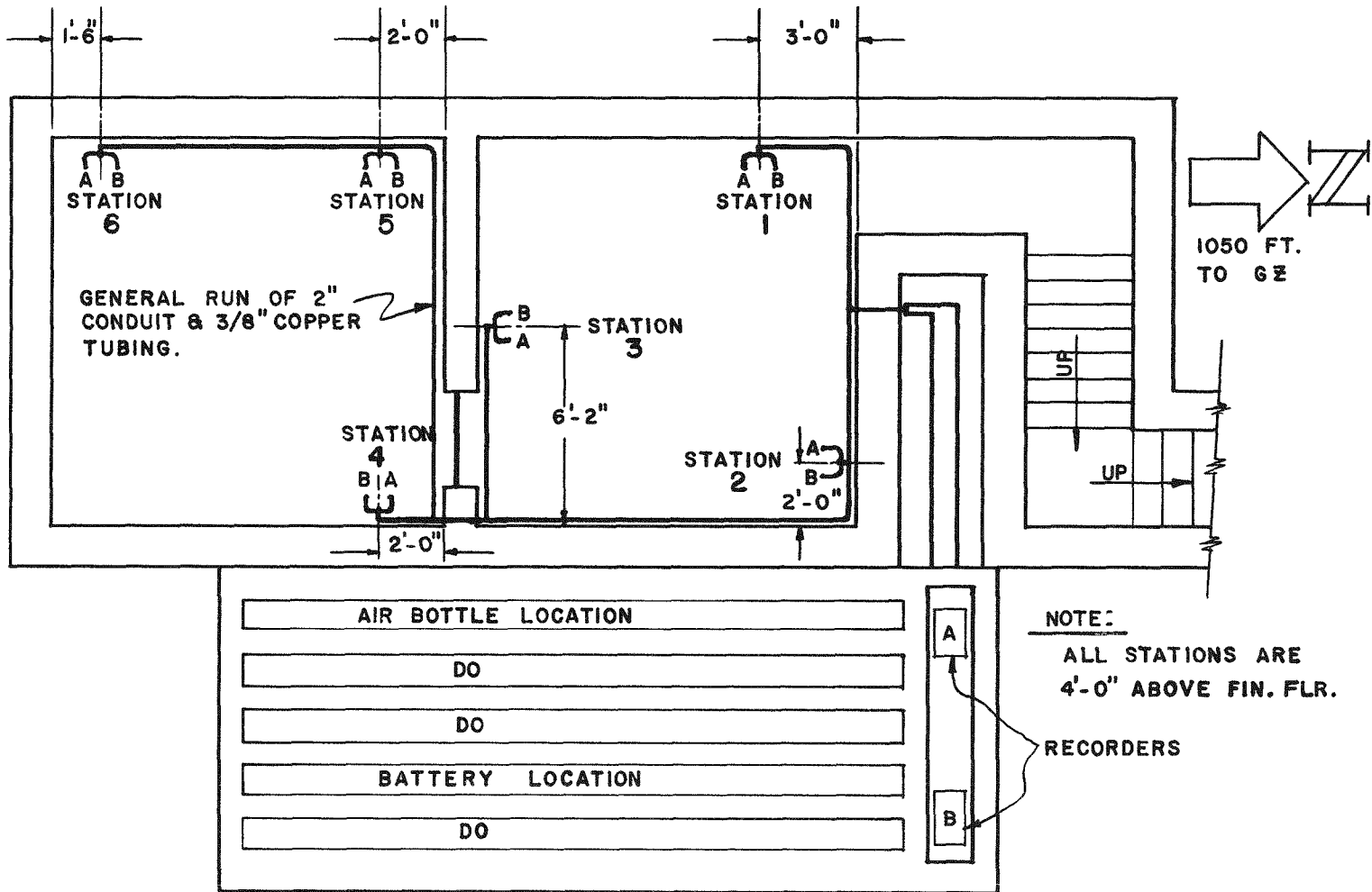
Fig. 2.1--Instrumentation lay-out, blast-biology shelter.
